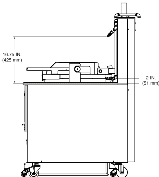
SIDE VIEW (NOZZLE LOCATION)
