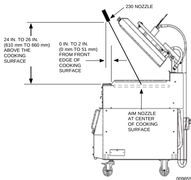
Broiler Side View
