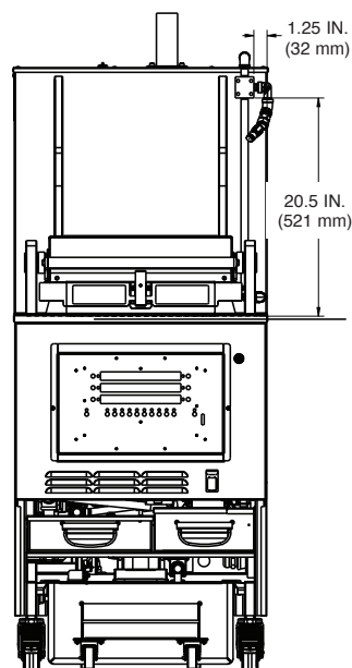
FRONT VIEW (TEE BLOCK LOCATION)
